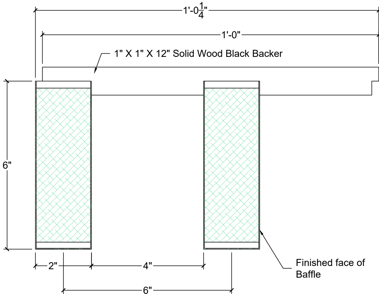
Typical Panel Section View
