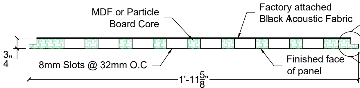
B P3 Panel Section View
