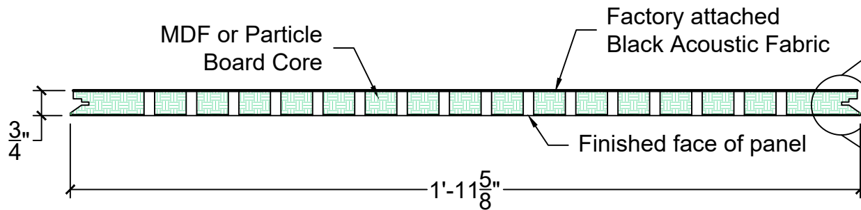
A P3 Panel Section View
