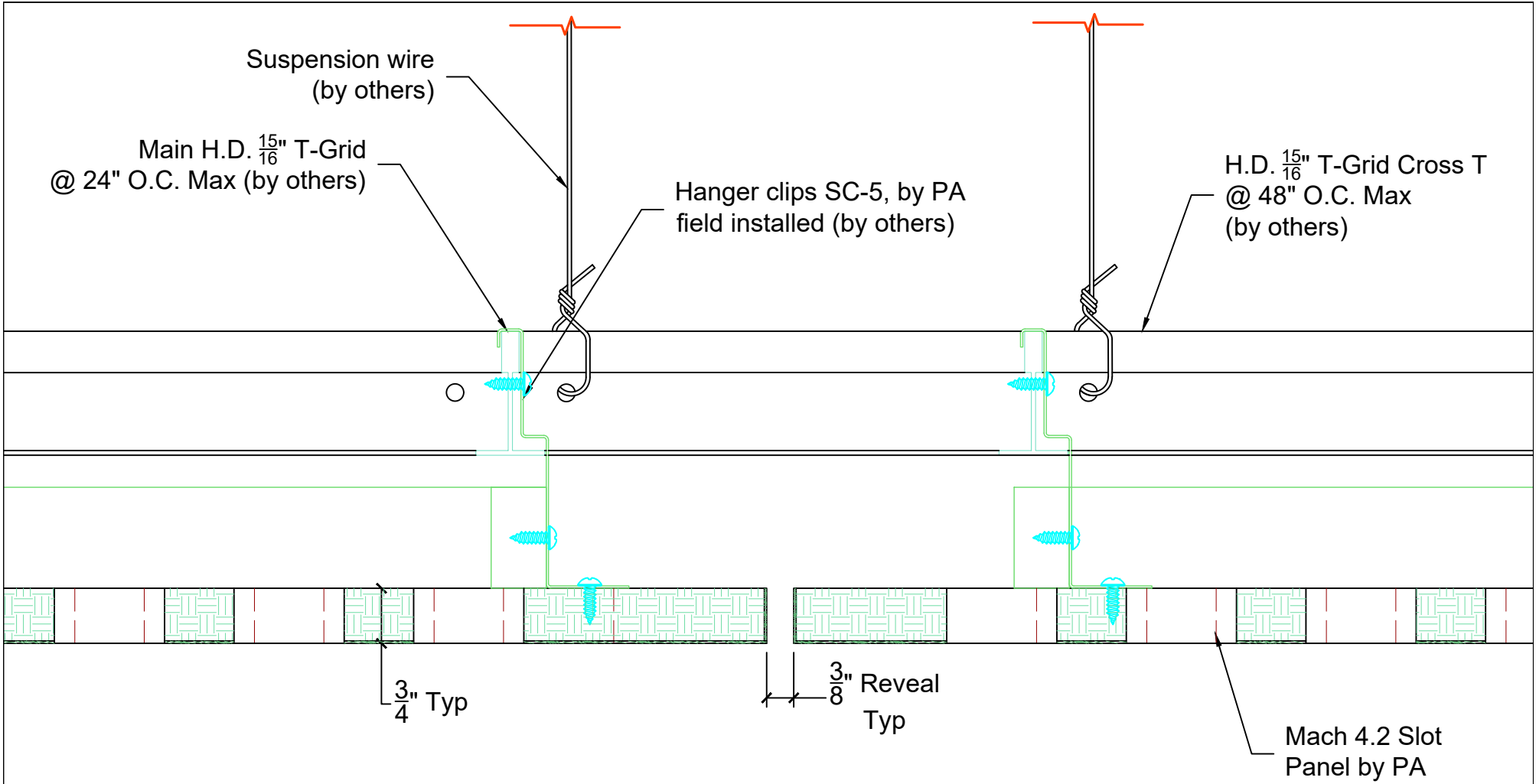
Panel Installation - Reveal between panels
