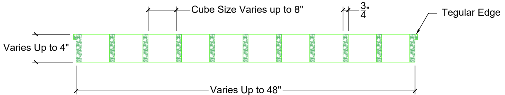
Tegular Edge Panel Section View
